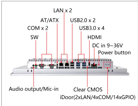
Default I/o View
