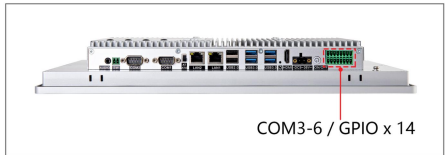
Optional I/O View : iDOOR-4x COM / 14xGPIO
